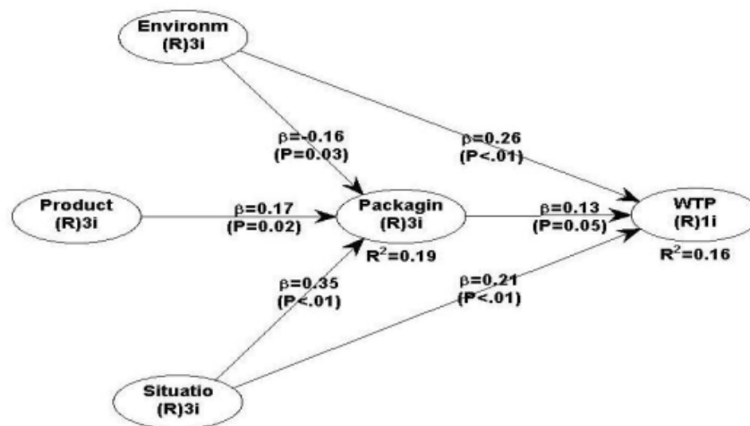
Fig. 1. The result of PLS-SEM.
