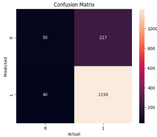
Fig. 3 Confusion Matrix with GridSearchCV
