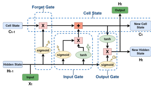
Gambar 2 Arsitektur Long Short - Term Memory
