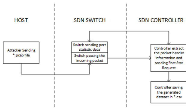
Fig. 4. Dataset extraction process
