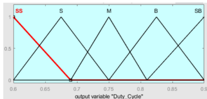
Gambar 5 Memberfunction Output Duty Cycle
