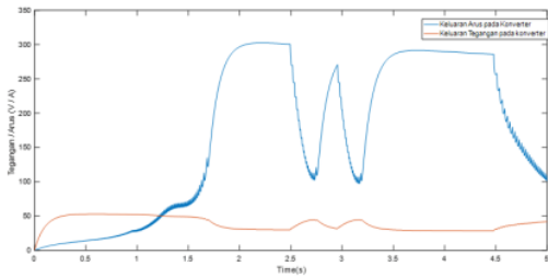
Gambar 13. Respon Arus/Tegangan Konverter Buck-Boost
