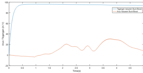
Gambar 12. Respon Arus/Tegangan Konverter Buck-Boost
