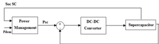
Gambar 7. Diagram Blok Power Management Strategy
