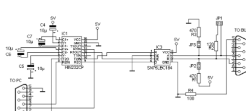
Gambar 2. Rangkaian Konverter RS485 to RS232
