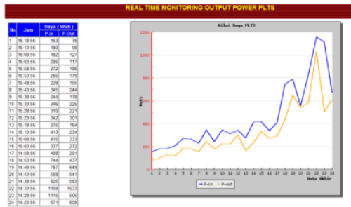
Gambar 11. Real Time PLTS
