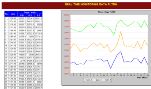
Gambar 12. Real Time PLTMH
