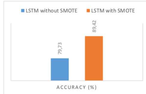
Figure 5. Comparison of the Effects of Using SMOTE
