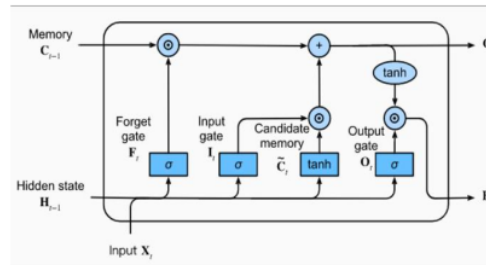
Figure 4. LSTM Architecture
