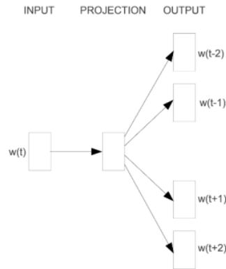
Figure 3. Illustration of the Skip-gram
