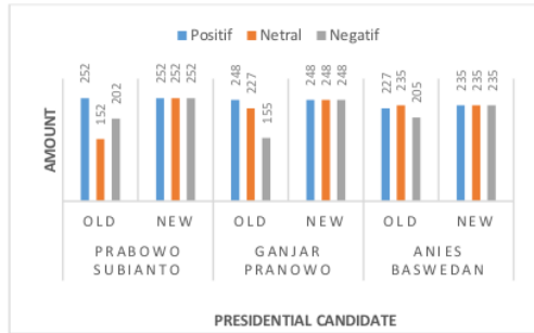
Figure 2. SMOTE Result
