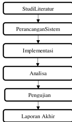
Gambar 1. Alur Penelitian
