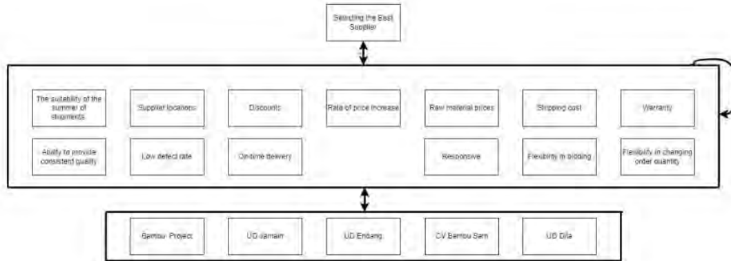
Figure 3. Network Structure of ANP
