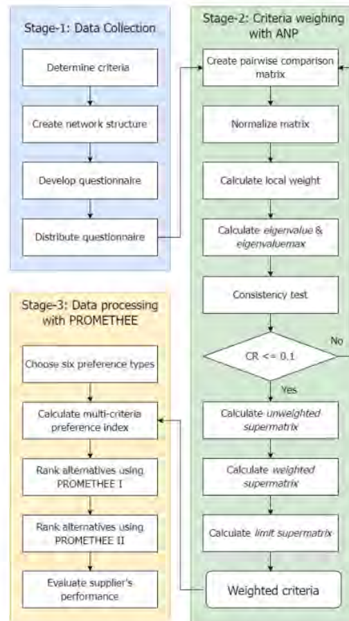
Figure 1. Integration of ANP and PROMETHEE on supplier performance evaluation
