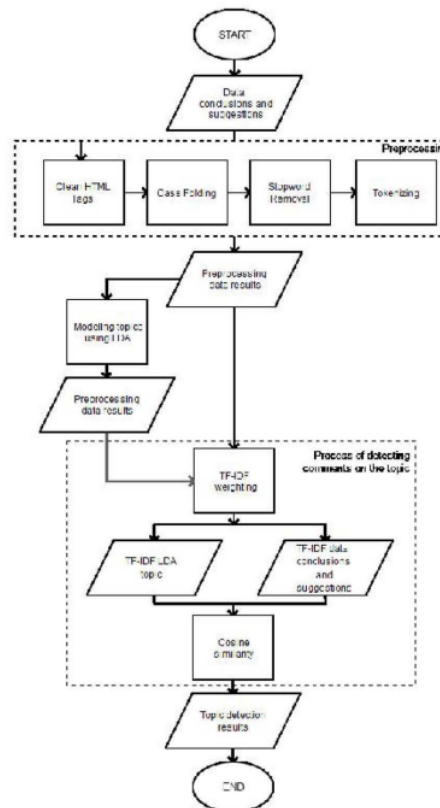
Fig. 1. Detection of reference topics and suggestions system
