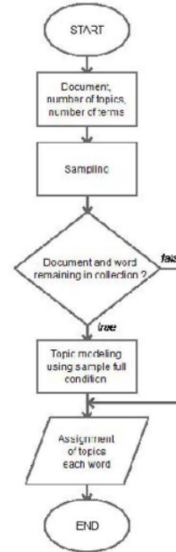
Fig. 2. LDA-based topic modelling process
