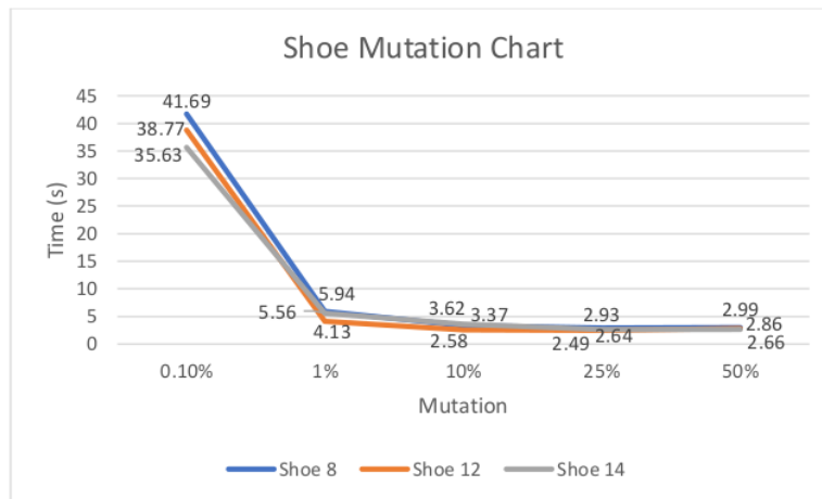
Figure 6. Mutation Probability Comparison Chart
