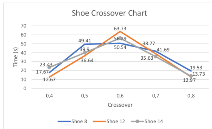
Figure 5. Crossover Probability Comparison Chart
