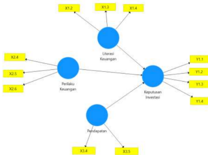
Gambar 3. Hasil Partial Least Square (PLS)
