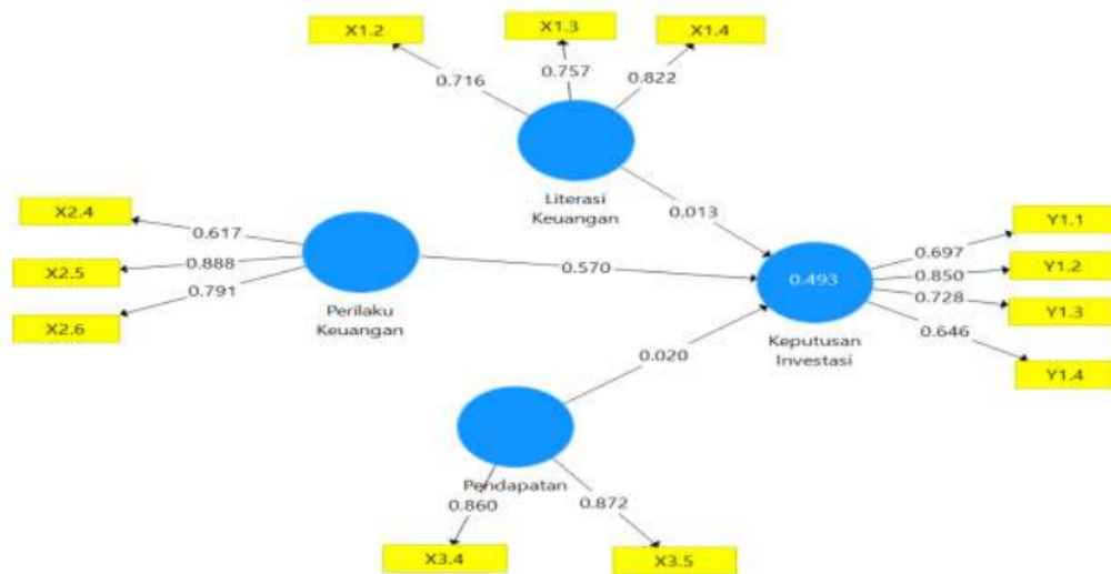
Gambar 4. Hasil Bootstrapping PLS
