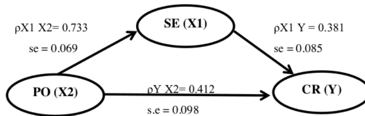
Figure 1: The path model
