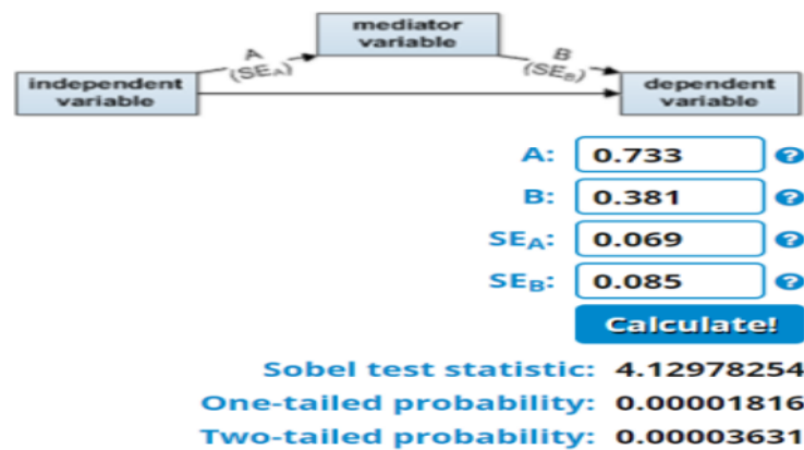
Figure 2. Output Sobell test online calculator model
