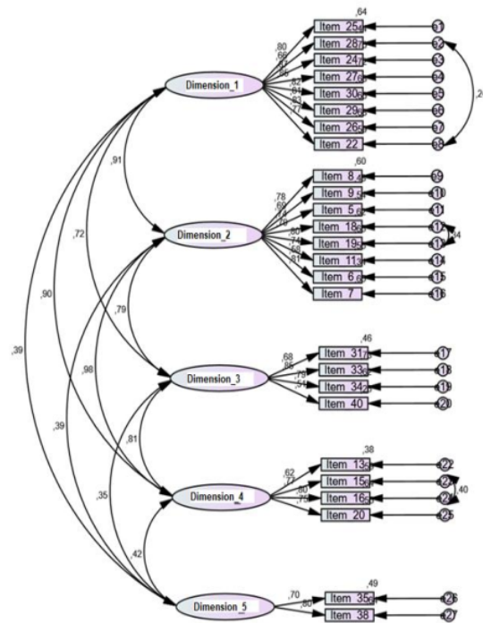
Figure 1. Results of confirmatory factor analysis (CFA Results)
