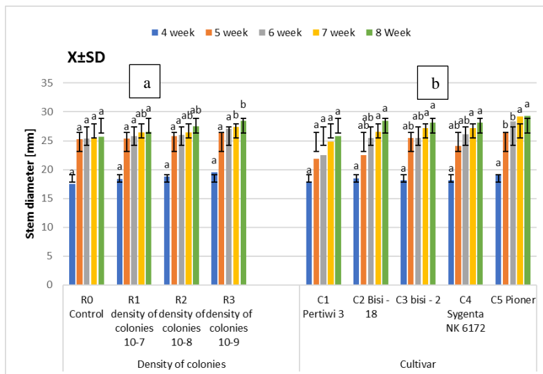
Fig. 2. (a) The average diameter of maize stem at DRC treatment, (b) the average diameter of maize stem at cultivar treatment.
