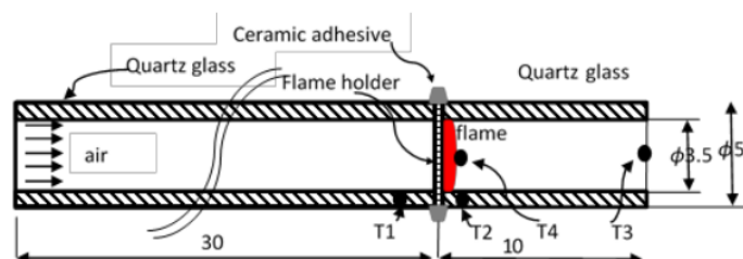
Figure 1. Mesocombustor and temperature measurement spot
