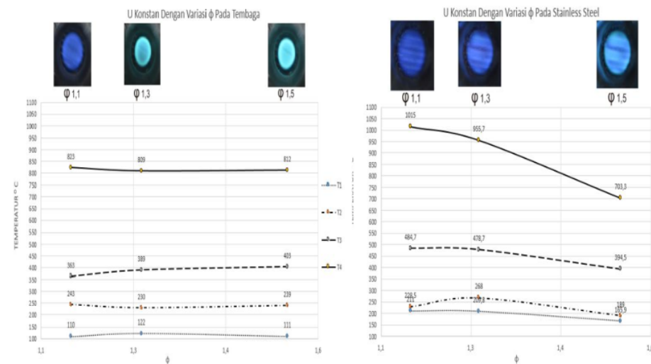
Figure 5. Flame visualization in U 38 cm/s with varied equivalence ratio ( \phi )
