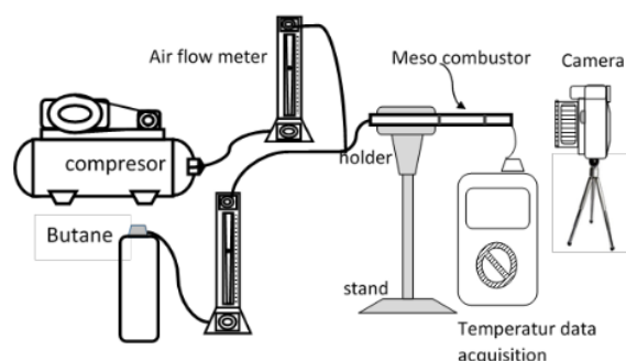
Figure 2. Experiment Installation Scheme
