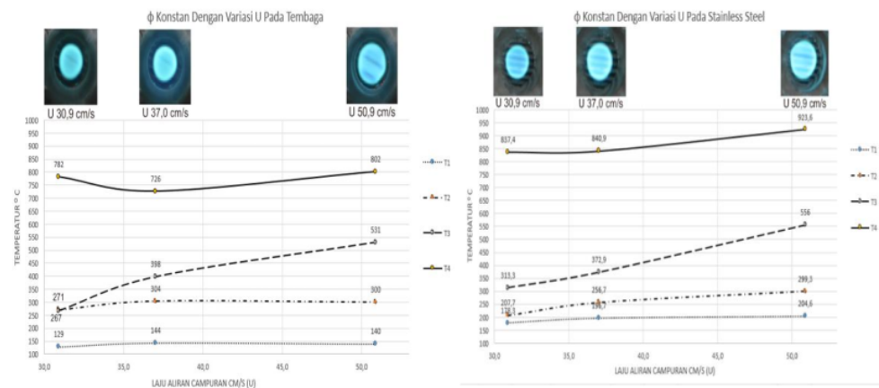
Figure 4. Flame visualization in \phi 1,3 with varied mixture flow velocity (U)
