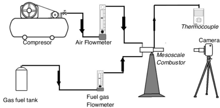
Fig. 4. Research installations for gas fuel
