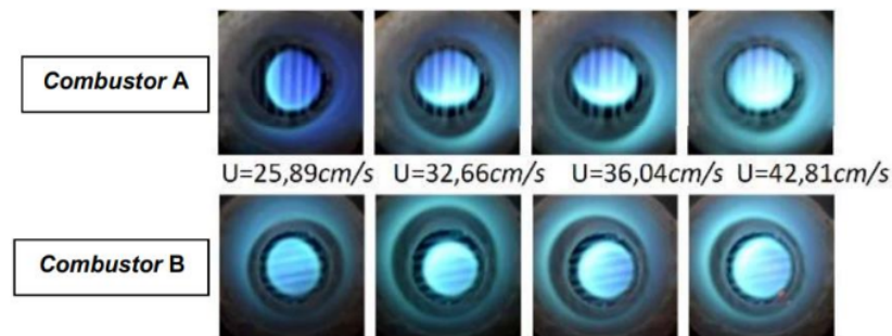
Fig. 8. Visualization of butane combustor flames A and B, at \phi = 1.03
