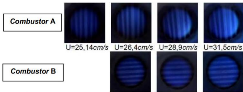
Fig. 6. Visualization of combustor hexane flames A and B, at \phi = 0.87
