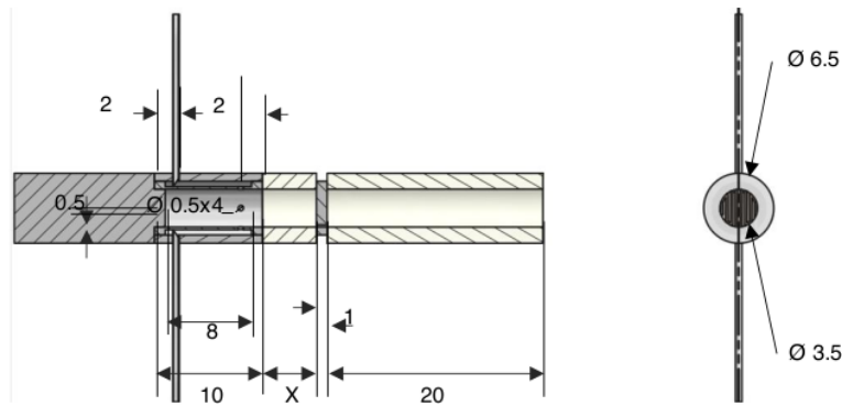
Fig. 2. Combustor B (unit: mm)
