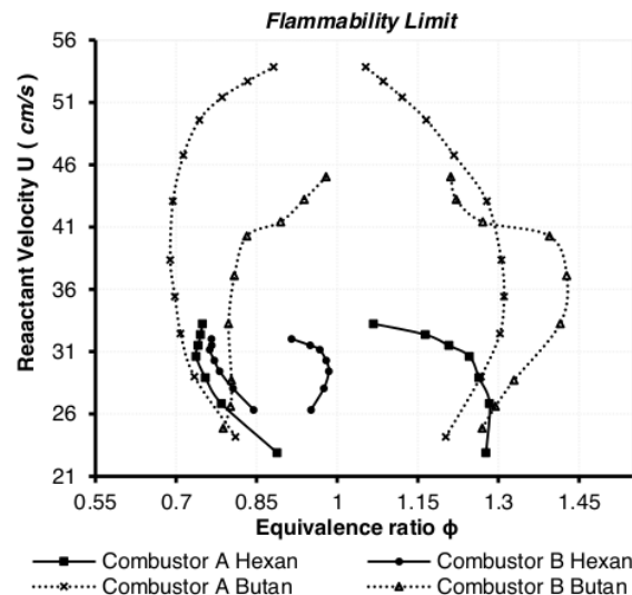
Fig. 5. Combustor flame stability A and B
