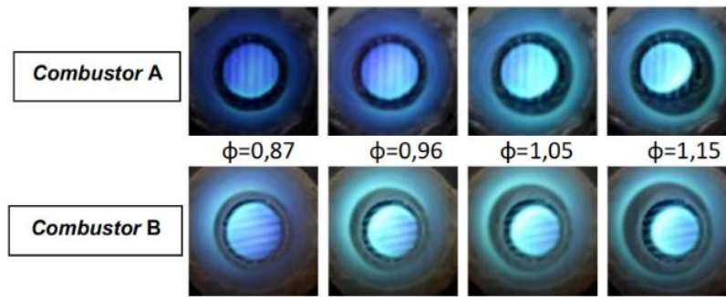
Fig. 9. Visualization of butane combustor flames A and B, at U=38.57 cm/s
