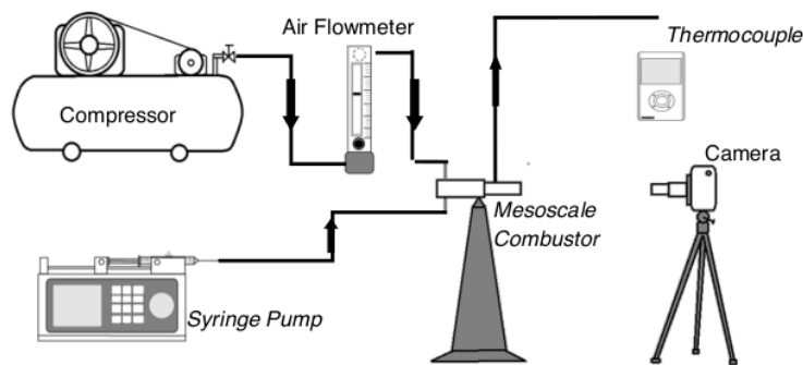
Fig. 3. Research installations for liquid fuel
