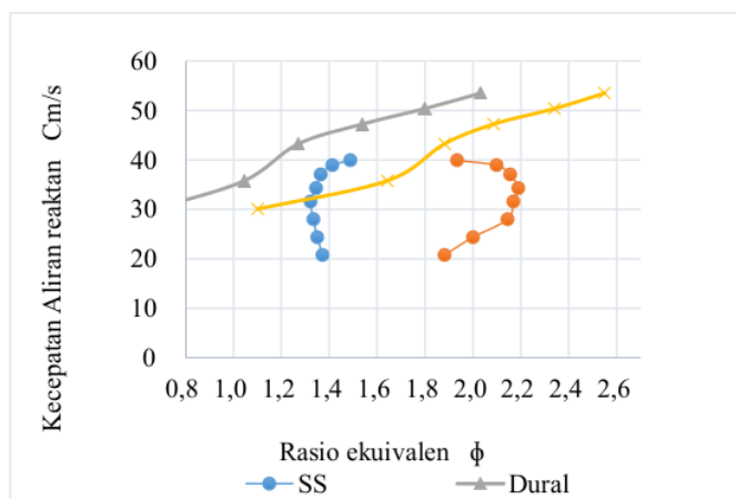
Gambar 8 Flammability limits .
