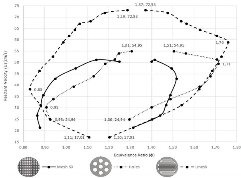
Fig. 3. Flammability limit
