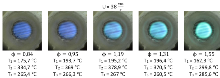
Fig. 10. Mesoscale flame visualization – combustor lines perforated plate on U = \text{constant} (front side)
