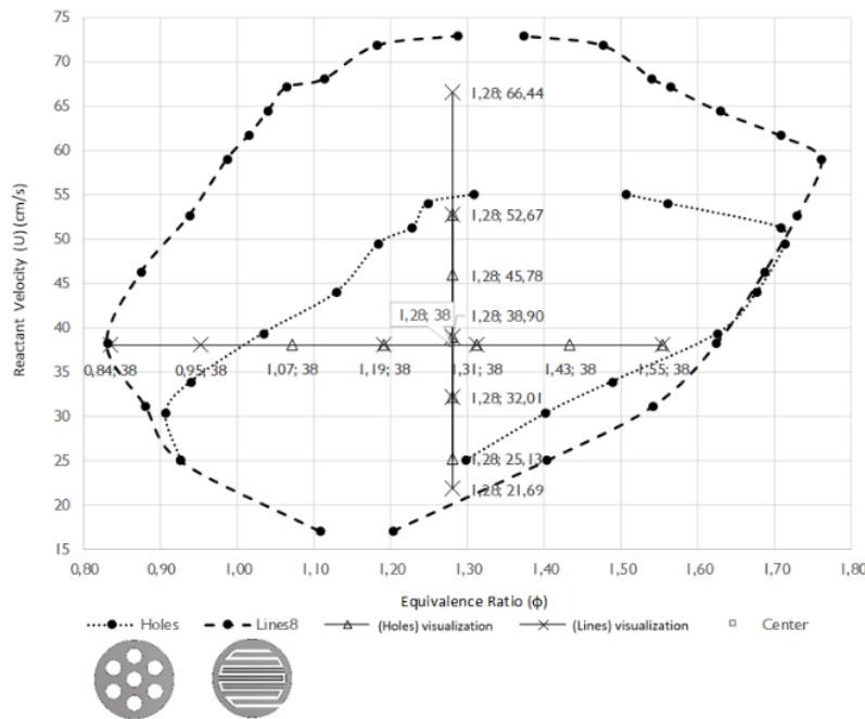
Fig. 4. Flammability limit for visualization take point and flame temperature
