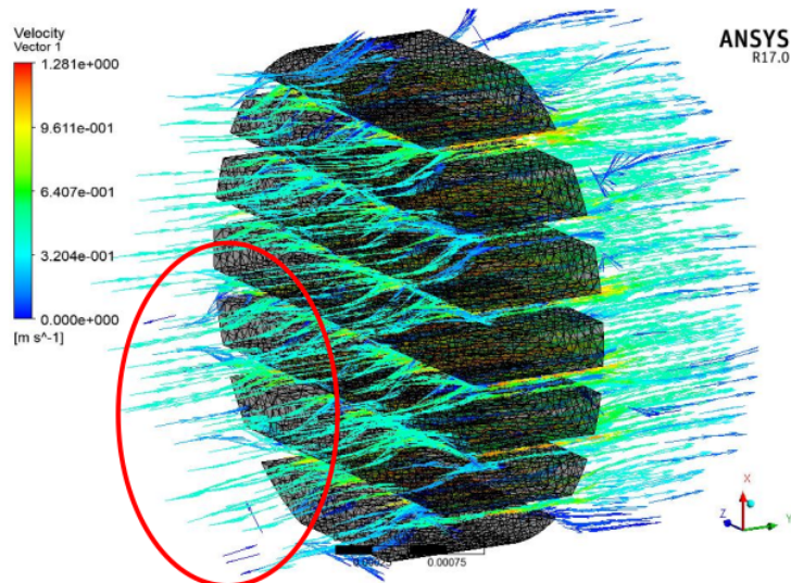
Fig. 12. Isometric view of the inlet combustor flame holder lines
