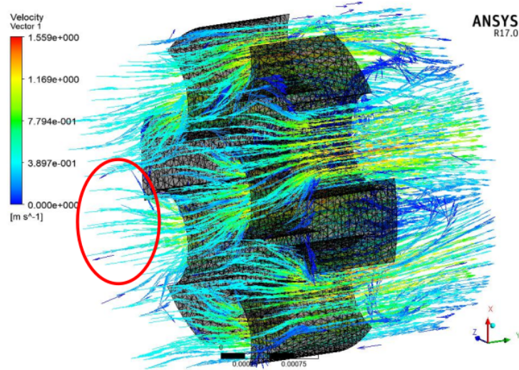
Fig. 11. Isometric view of the inlet combustor flame holder holes
