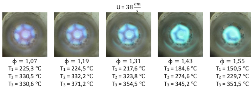
Fig. 9. Mesoscale flame visualization – combustor holes perforated plate on u constant (front side)
