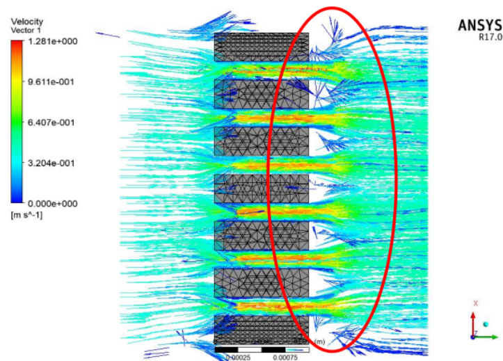
Fig. 14. Side view of the combustor flame holder lines
