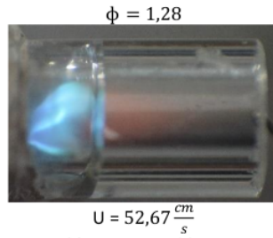
Fig. 6. Visualization of perforated plate flame holes at \phi = 1,28 and U = 52.67 \text{ cm/s} (side side)
