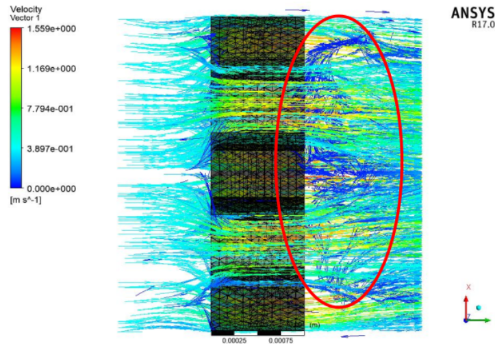
Fig. 13. Side view of the combustor flame holder holes
