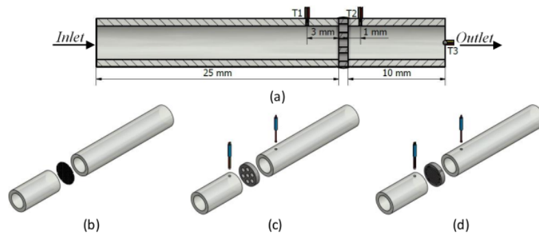
Fig. 1. Meso-combustor (a) Technical drawing of mesoscale combustor (b) Wire mesh meso scale combustor (c) Holes perforated plate meso scale combustor (d) Lines perforated plate meso scale combustor
