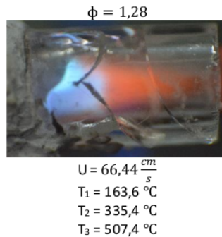
Fig. 8. Mesoscale flame visualization – combustor lines perforated plate on \phi constant (side-side)
