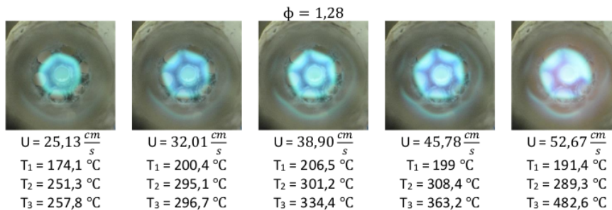
Fig. 5. Mesoscale flame visualization – combustor holes perforated plate on \phi = 1,28 and U varies (front side)
