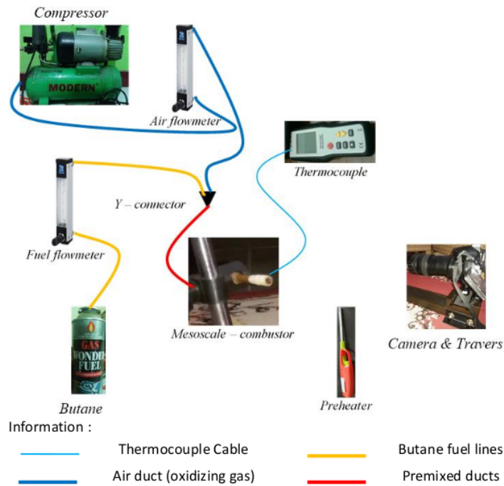
Fig. 2. Research installation scheme
