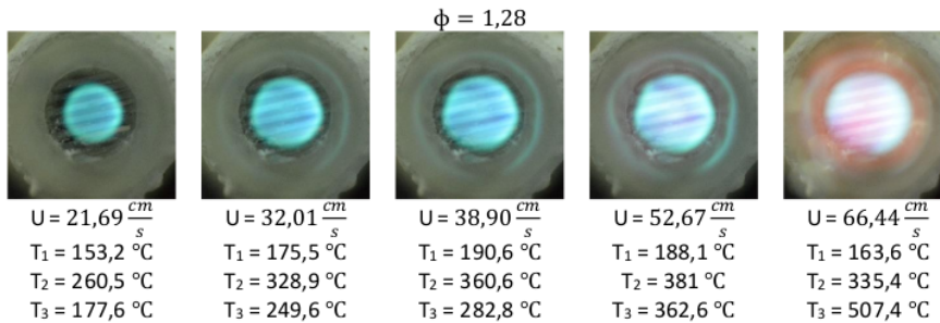
Fig. 7. Mesoscale flame visualization – combustor lines perforated plate on \phi constant (front side)
