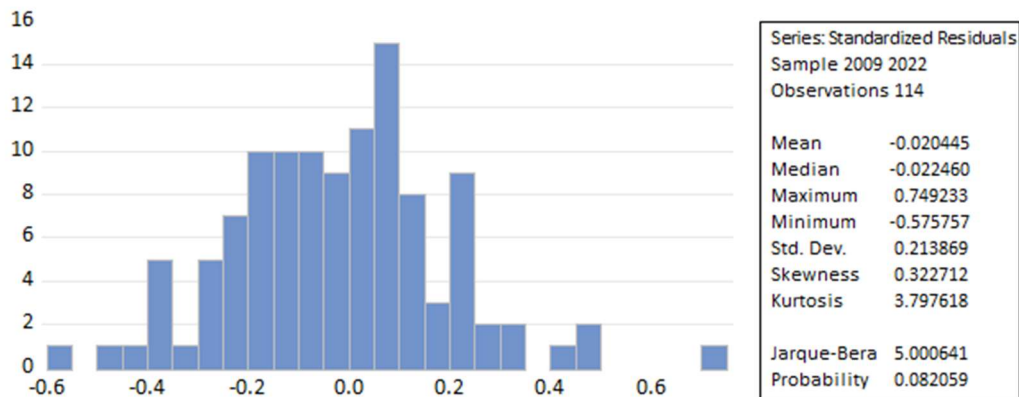
Figure 1 Normality Test
