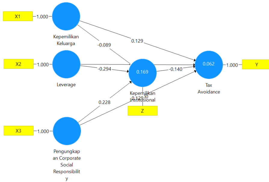
Figure 1.1 PLS Algorithm
