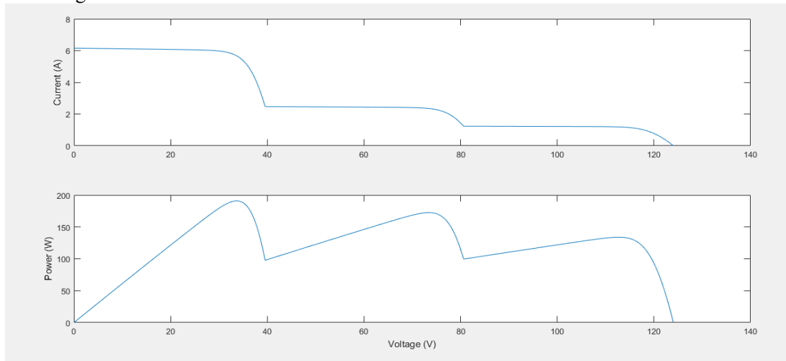
Figure 6. I-V and P-V curves in partial shading conditions
