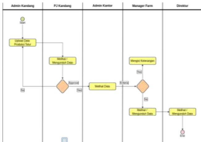
Gambar 3. Activity Diagram
