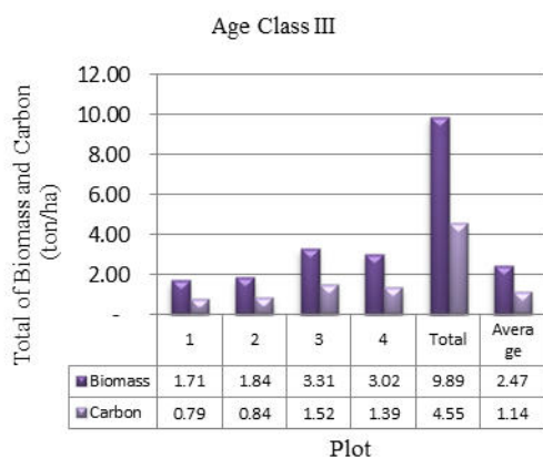
Figure 4. Biomass and Carbon of Under-growing plants from age class I to IV
