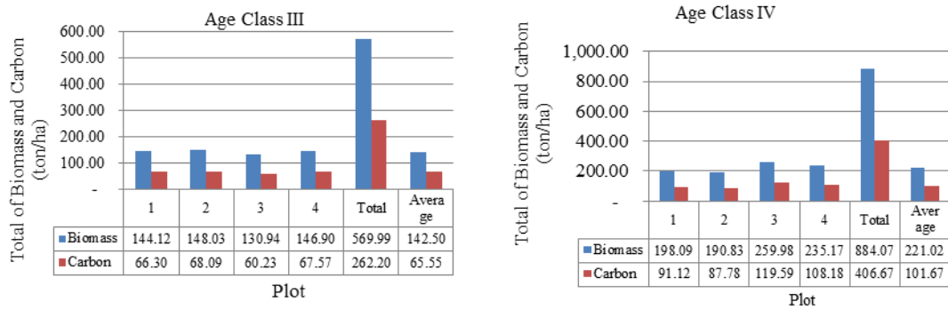
Figure 1. Biomass and Carbon of Teak Plantation in Age Class I – IV
