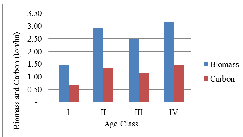
Figure 6. The average total of under-growing plant's carbon from age class I to IV
