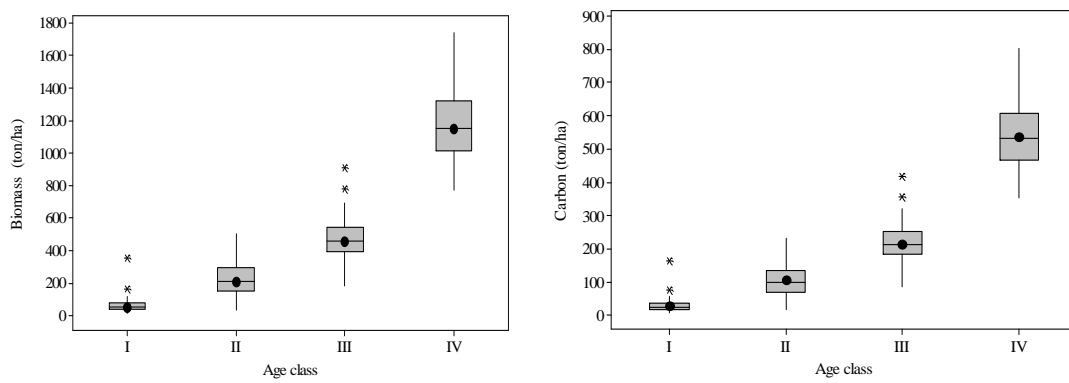
Figure 2. Total of Biomass and Carbon of Teak Plantations in Age Class I – IV
