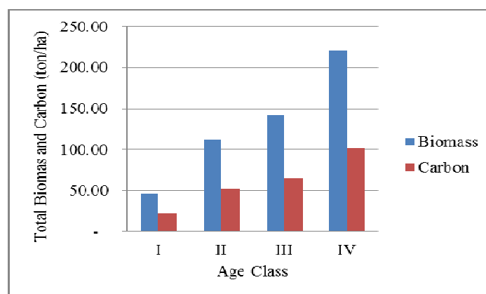
Figure 3. Graph of the total average of Biomass and Carbon of Teak Plantations from age class I to IV
