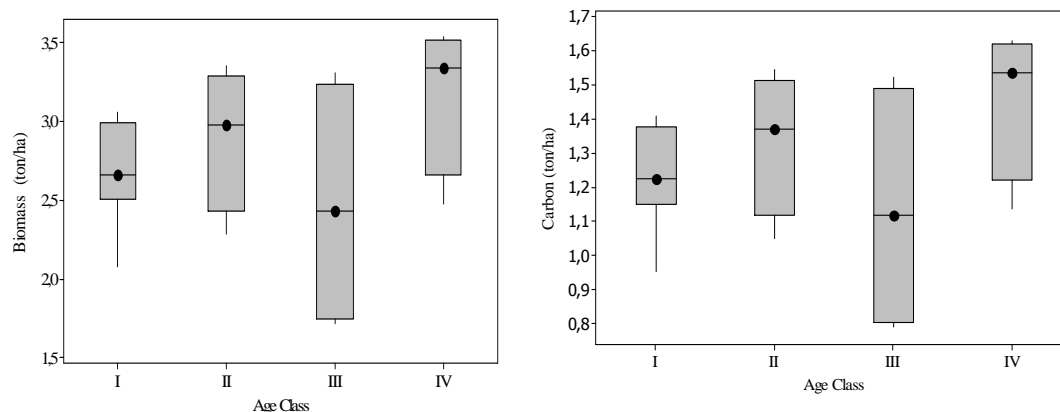
Figure 5. Total of Biomass and Carbon of under-growing plants from age class 1 to IV
