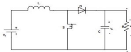
Figure 4. DC-DC boost converter circuits
