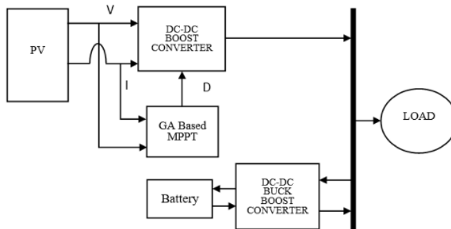
Figure 2. Block diagram of solar system
