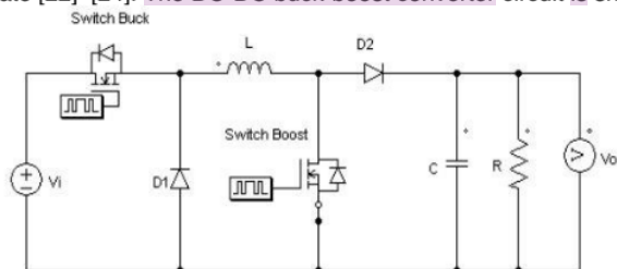
Figure 5. DC-DC buck boost converter
