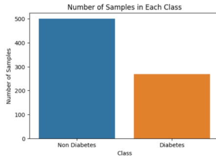
Fig. 2 Before Resampling
