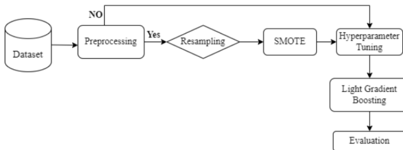
Fig. 1 Research Flow
