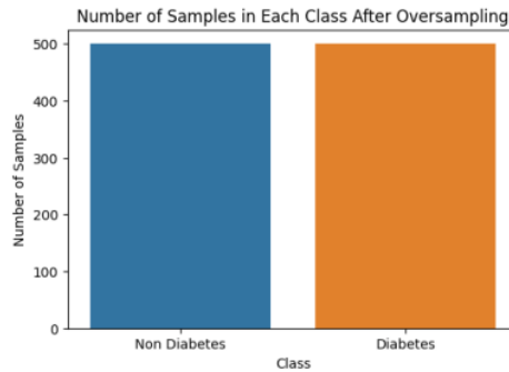
Fig. 3 After Resampling
