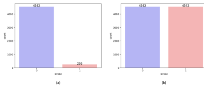
Figure 5. Number of samples for the dataset, (a) before resampling, and (b) after resampling
