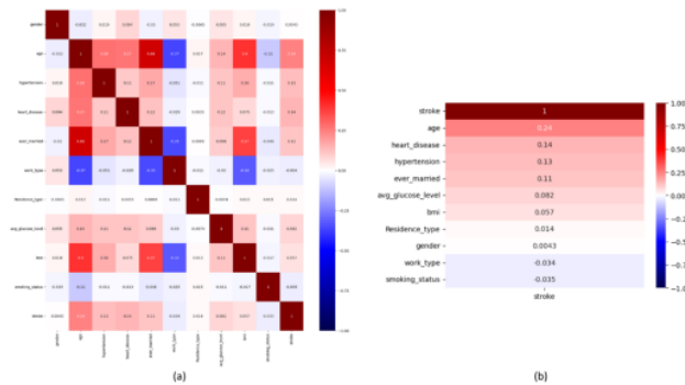
Figure 4. (a) Correlation matrix between features, and (b) correlation with target classq
