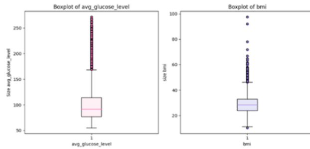
Figure 2. Data before handling outliers
