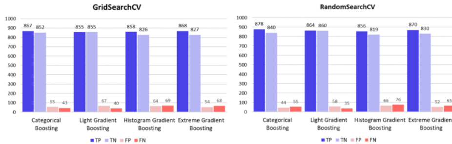
Figure 6. Comparison of confusion matrix in graph
