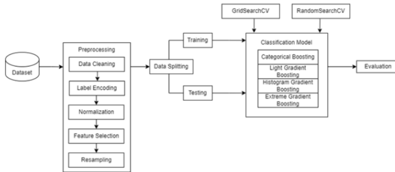
Figure 1. Research Methodology
