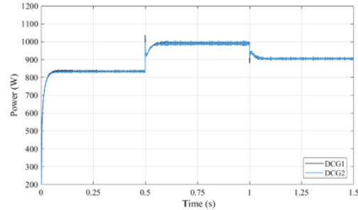
Fig. 12. Output power of the DCG with Fuzzy-PI
