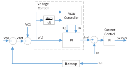
Fig. 4. The proposed control block diagram of droop control
