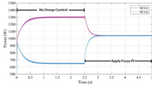
Fig. 10. Dynamic response of system with Fuzzy-PI
