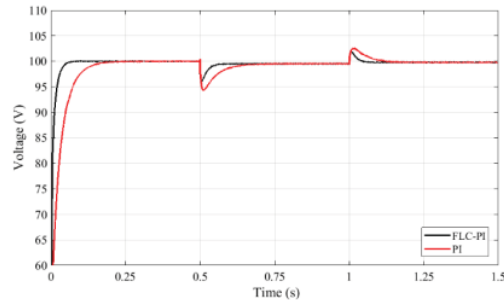
Fig. 13. Voltage comparison of droop control under load change
