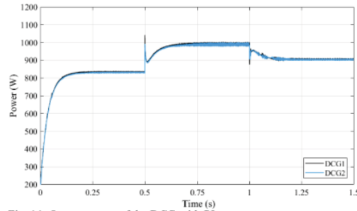
Fig. 11. Output power of the DCG with PI
