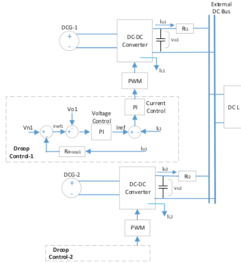
Fig. 2. Droop Control Architecture for DCMG
