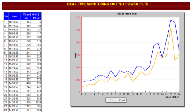
Gambar 11. Real Time PLTS
