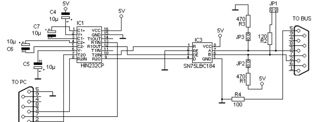
Gambar 2. Rangkaian Konverter RS485 to RS232
