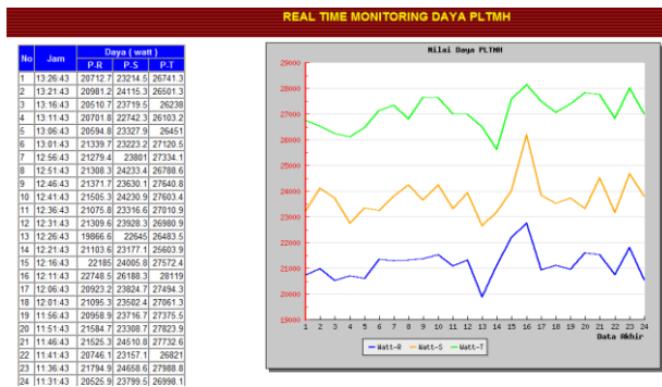
Gambar 12. Real Time PLTMH
