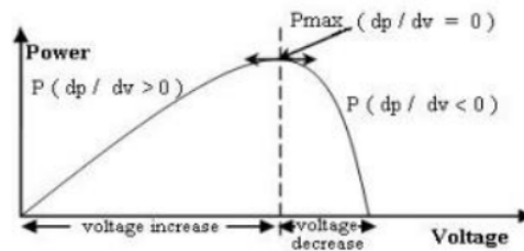
Figure 3. Power-voltage characteristic of a PV module
