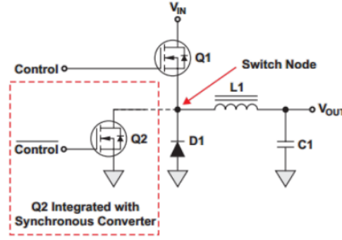
Figure 4. Synchronous and nonsynchronous buck circuits
