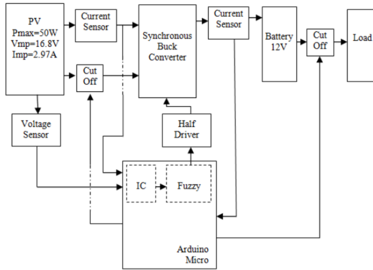
Figure 1. Photovoltaic with MPPT system
