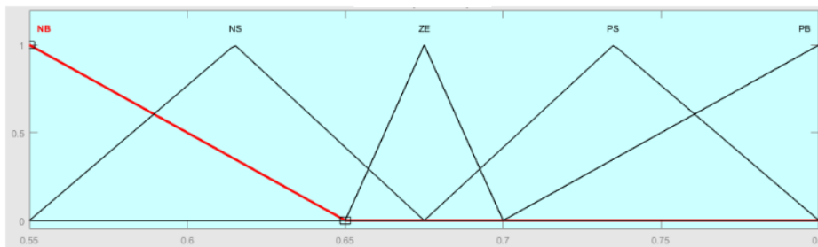
Figure 8. Member function of duty cycle
