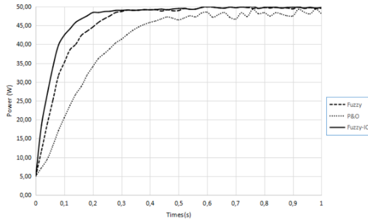
Figure 10. Result of MPPT implementation with various algorithms
