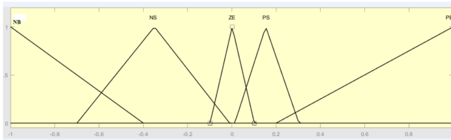
Figure 6. Membership functions of dI/dV
