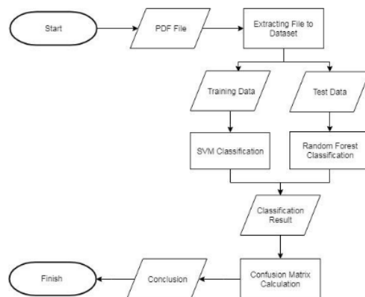
Figure 2. The flow of Research Methods
