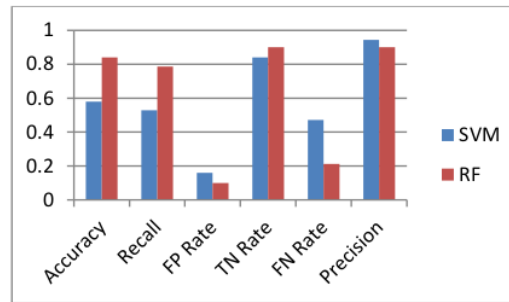
Figure 5. Results of Comparison in the Form of Graphs
