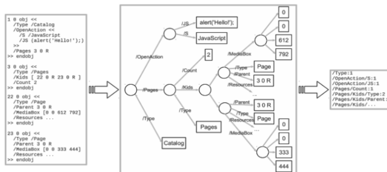
Figure 3. PDF Structure Representation
