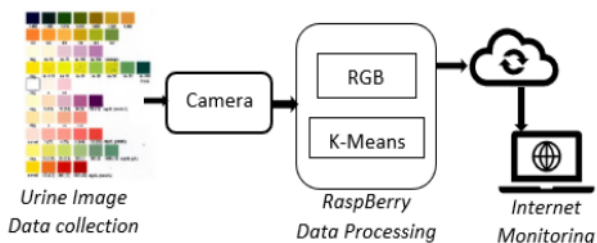
Fig. 1. Illustrated hardware and software design
