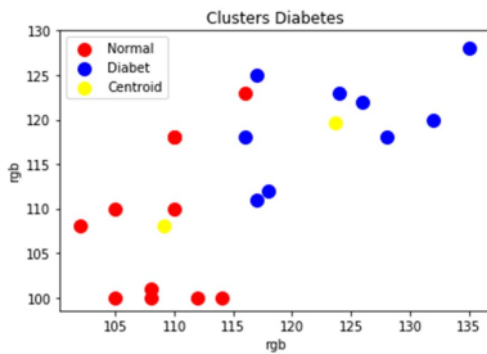
Fig. 4. Clustering chart result
