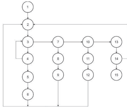
FIGURE 6. Flowgraph of AR Reog Ponorogo
