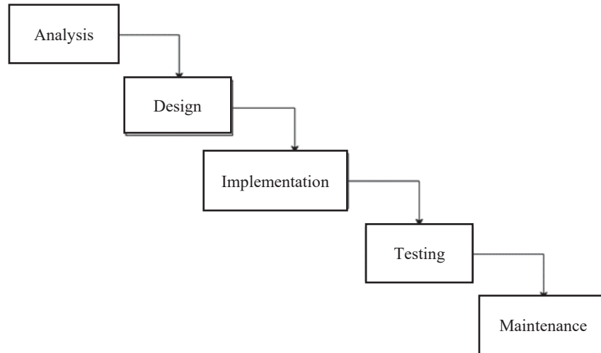
FIGURE 1. Waterfall Model [7]
