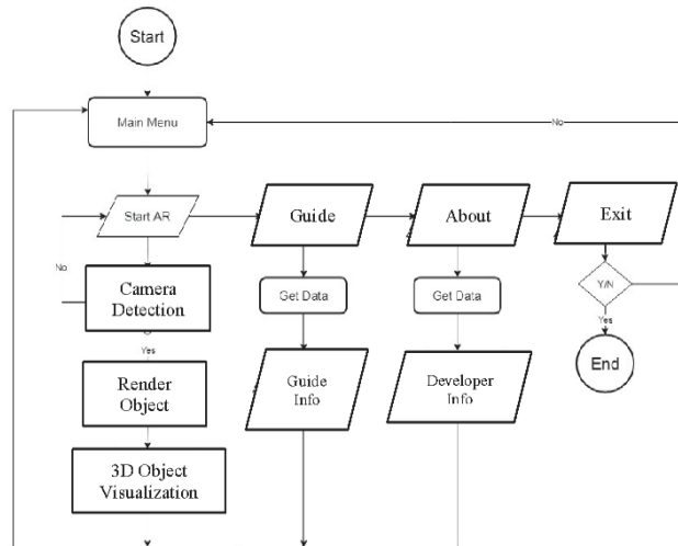
FIGURE 5. Flowchart of AR Reog Ponorogo
