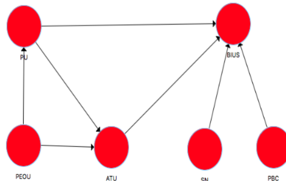
Gambar 2. Inner Model
