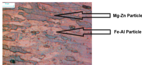
Figure 2. Microstructure of Al 7075 after HT
