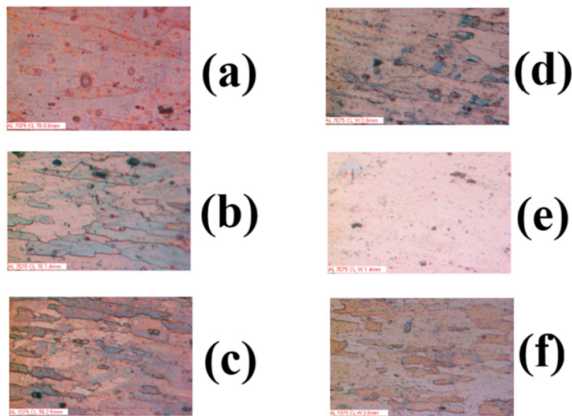
Figure 1. Microstructure of Al 7075 before and after HT
