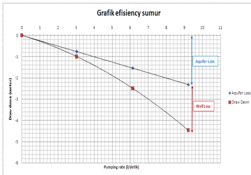
Gambar 12. Grafik Aquifer Loss dan Well Loss
