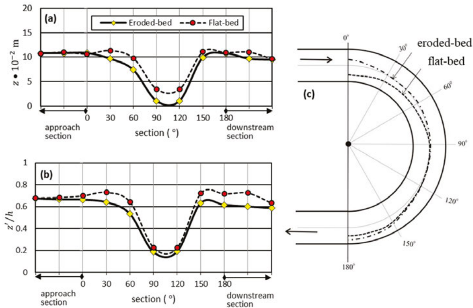
Fig. 10. Path of maximum velocity: a) based on elevation, b) based on relative distance, c) plan view; z = vertical distance from the bed, h = flow depth; source: own study
