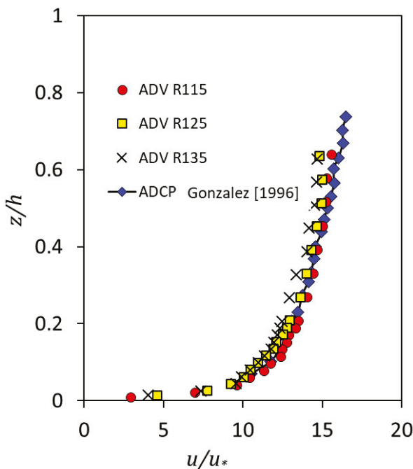
Fig. 3. Comparison of non-dimensional velocity ( u/u_* ) profile taken by Acoustic Doppler Velocimetry (ADV) vs. Acoustic Doppler Current Profilers (ADCP); z = vertical distance from the bed, h = flow depth; source: own elaboration
