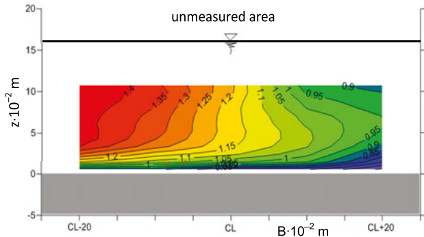
Fig. 8. Normalised longitudinal velocity ( u/U ) contours in downstream section; z = vertical distance from the bed; B = width of the channel; source: own study
