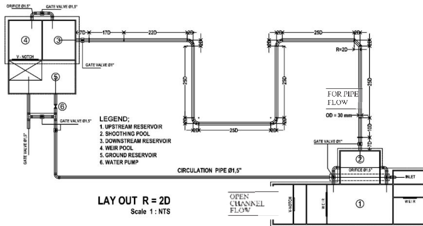
FIGURE 2. Plan model schematic for discharge calibration [14]
