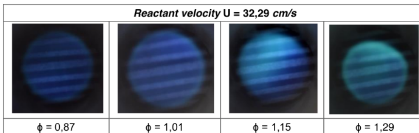
Figure 6. Flame visualization at constant reactant velocity
