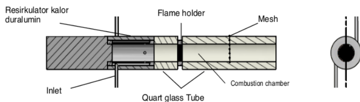
Figure 1. Structure of mesoscale combustor
