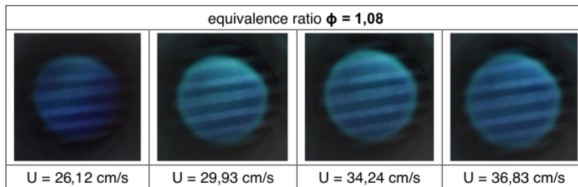
Figure 5. Flame visualization
