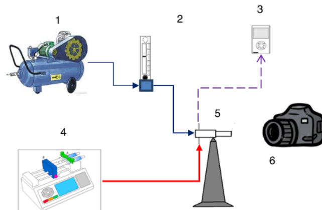
Figure 3. Research Installation 1). Compressor, 2). Air flow meter, 3). thermocouple, 4). Syringe pump 5). Meso combustor, 6). Camera
