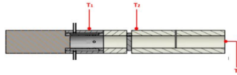
Figure 7. Temperature capture point
