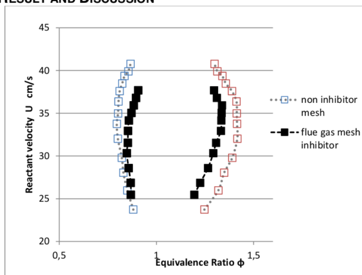
Figure 4. Flammability limits
