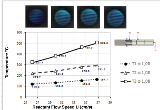
Figure 8. Flame temperature with a constant equivalent ratio
