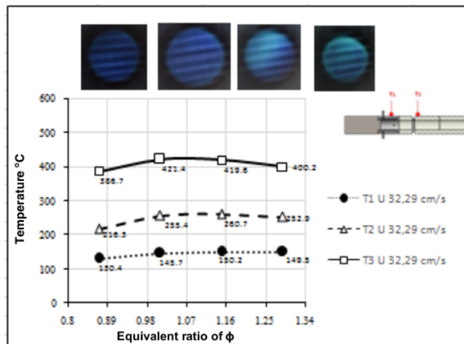
Figure 9. The flame temperature at a constant reactant flow velocity
