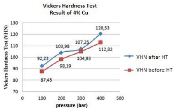
Figure 3. The graph of relationship between pressure squeeze casting with the Vickers test results of 4% cu composition
