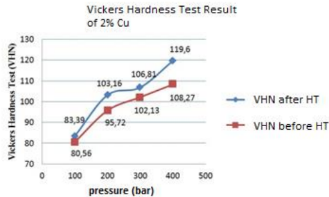
Figure 2. The graph of relationship between pressure squeeze casting with the Vickers test results of 2% Cu composition
