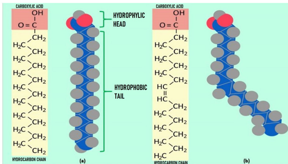
Figure 1. Fatty acid structures. 7 This compound is a carboxylic acid composed of long hydrocarbon chains with a chemical formula of \text{R}-\text{COOH} or \text{R}-\text{CO}_2\text{H} with a structure consisting of a hydrophilic head and a hydrophobic tail section.
