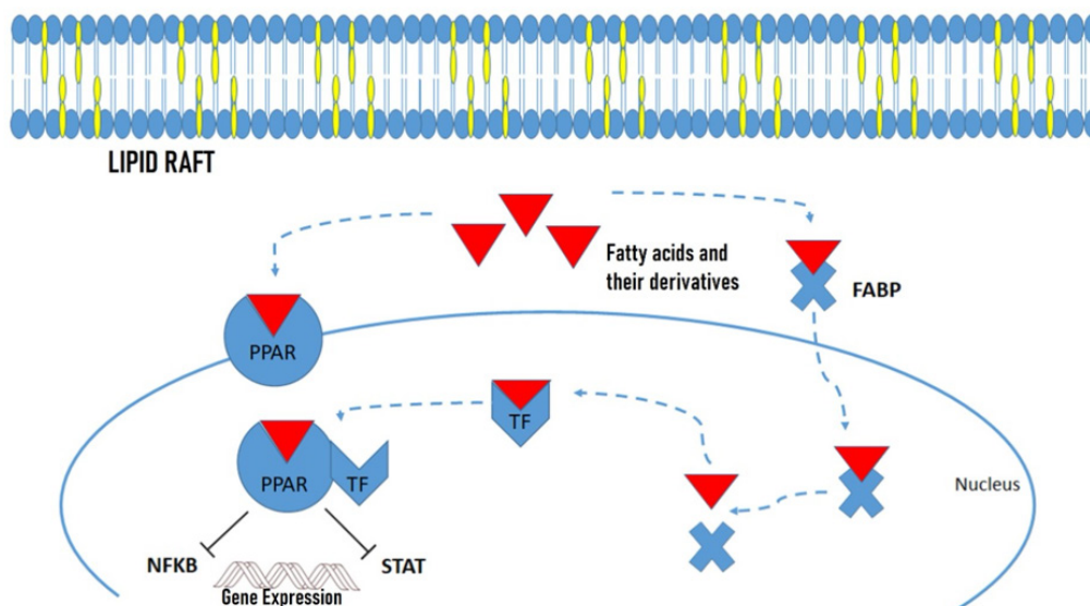
Figure 2. Fatty acid pathways in cell regulations. 10,15,16
