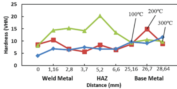
FIGURE 3. Relationship of Specimen Hardness to Point Distance
