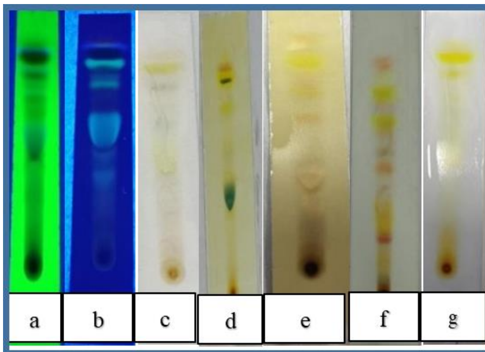
Figure 1. Chromatogram profile of ethyl acetate fraction of E. palmifolia separated over stationary phase of silica gel F_{254} by the mobile phase of ethyl acetate – chloroform, 3:7 (v/v), and visualized under (a) UV 254, (b) UV 365, as well as visible light after derivatization with (c) anisaldehyd-sulfuric acid, (d) Dragendorff’s reagent, (e) FeCl3, (f) KOH, and (g) 10% H2SO4
