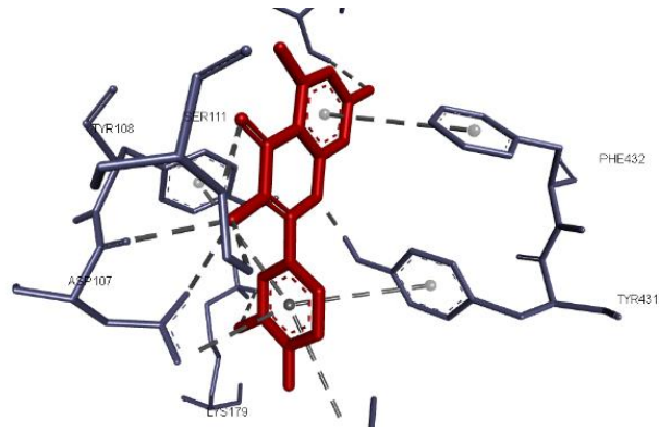
(a) Quercetin
