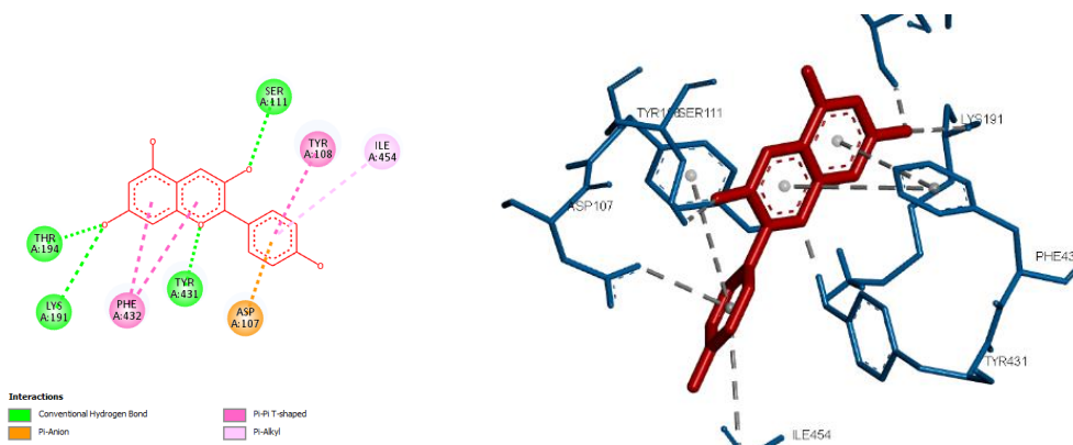
(c) Pelargonidin
